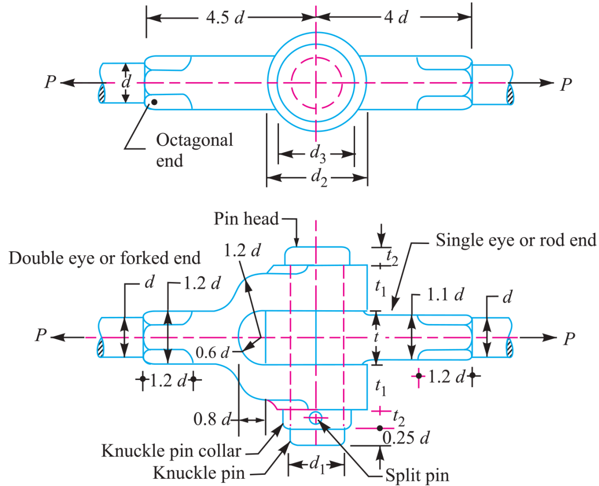
Fig. 12.16. Kunckle joint.
